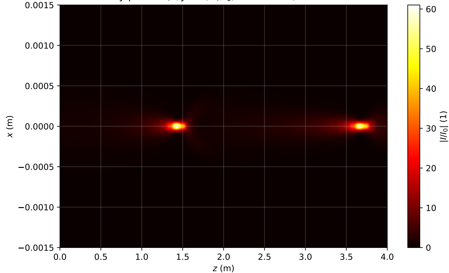
Intensity profile I(x, y = 0, z)/I_0 , P_{in}=1.7P_{cr} , artificial time
